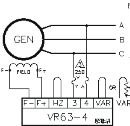
Interconnection Diagram, 208-240 V Nominal
